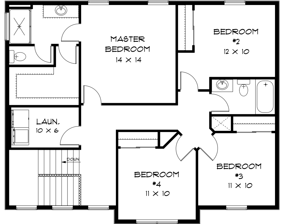
KINTZEL SECOND FLOOR PLAN 1090 SQ. FT.
